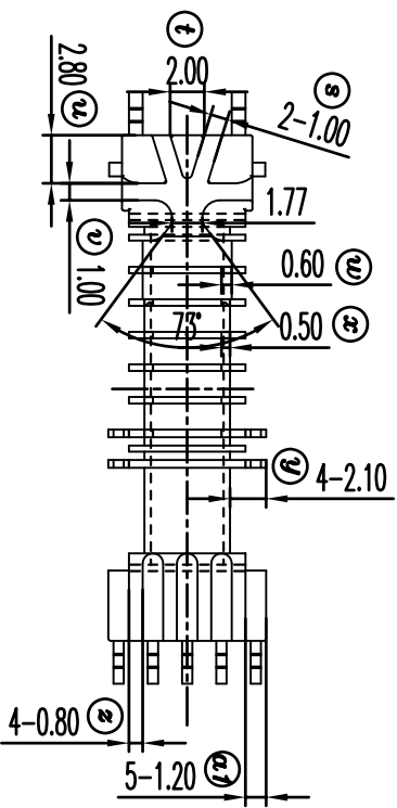
SECTION C-C
