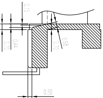
SECTION I-I
